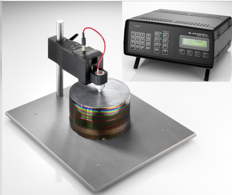
Multi Height Probe shown with AFPP Motorized Z Motion arm, Probing a Tall or Thick Material
