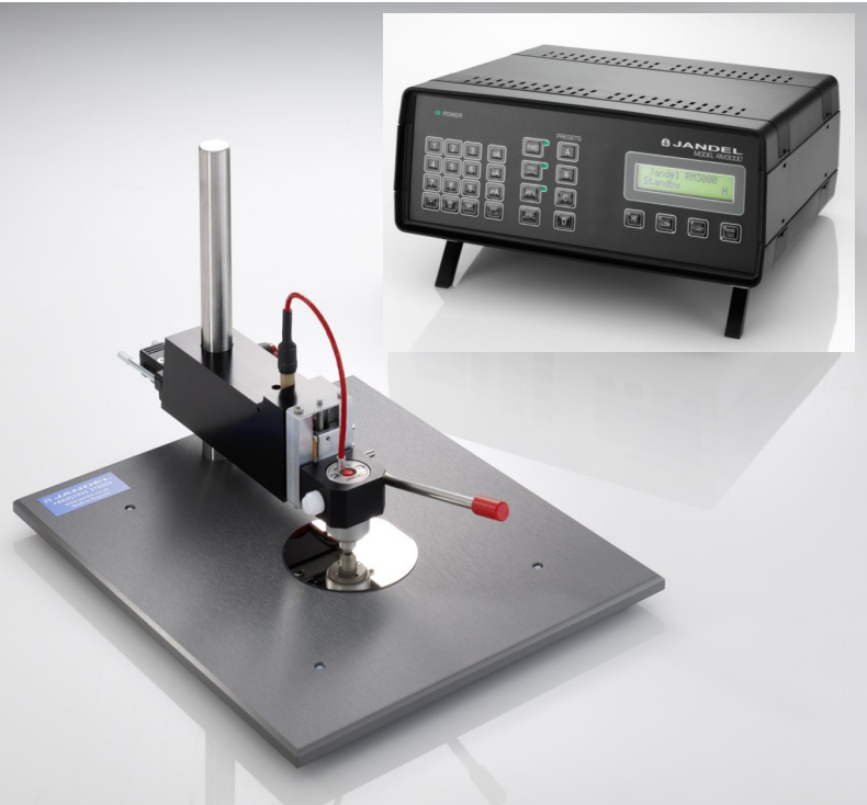
Multi Height Probe with Arm Lowered for Measuring a Flat Material
